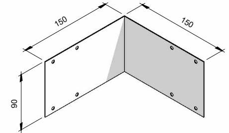
Detail Corner Plate
