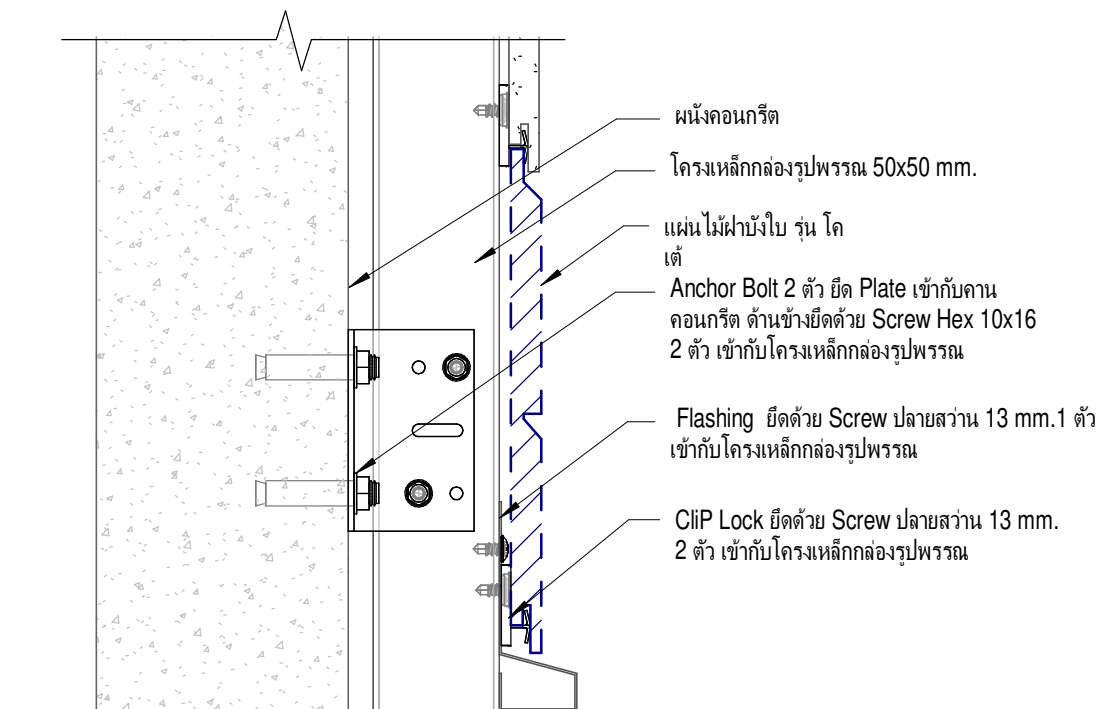
Section View
