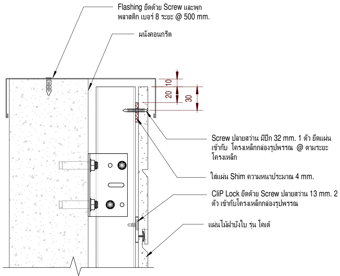
Section View
