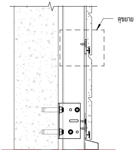
Section
