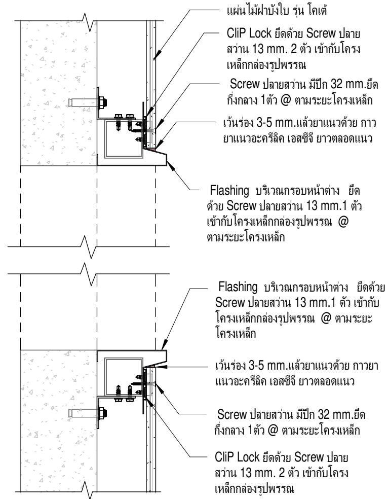
Section 1
