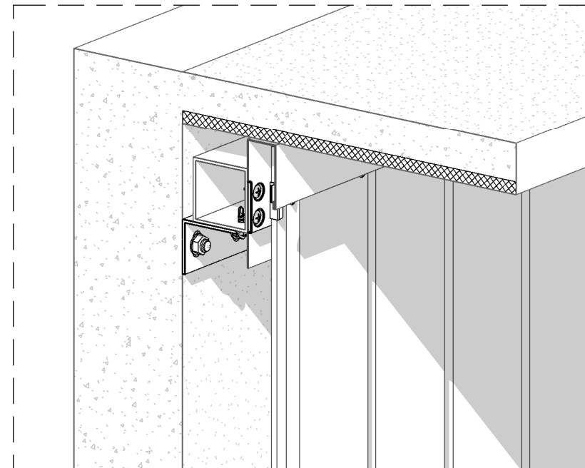
3D View
