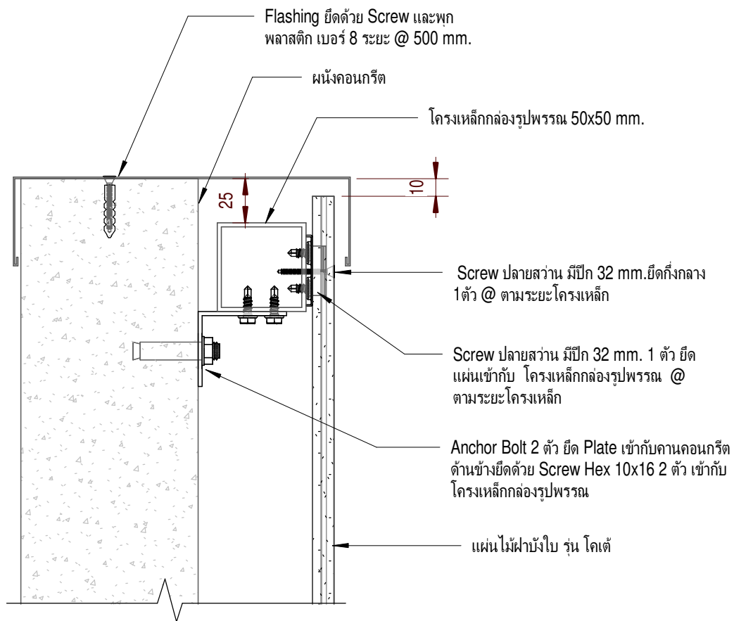
Section View
