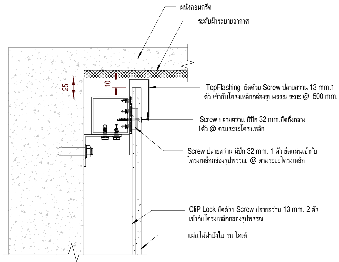
Section View
